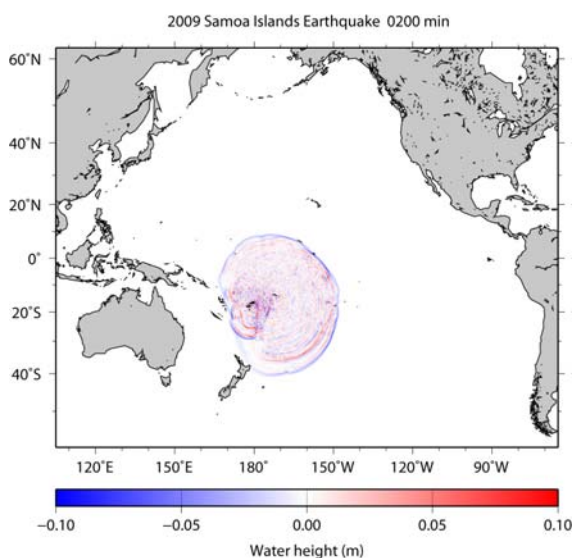
Tsunami simulation
