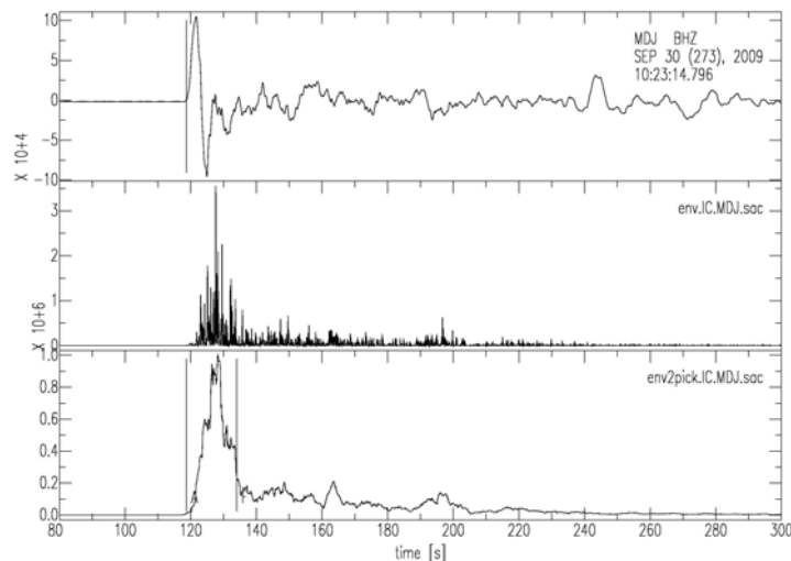
Example of measurements of high frequency energy radiation
