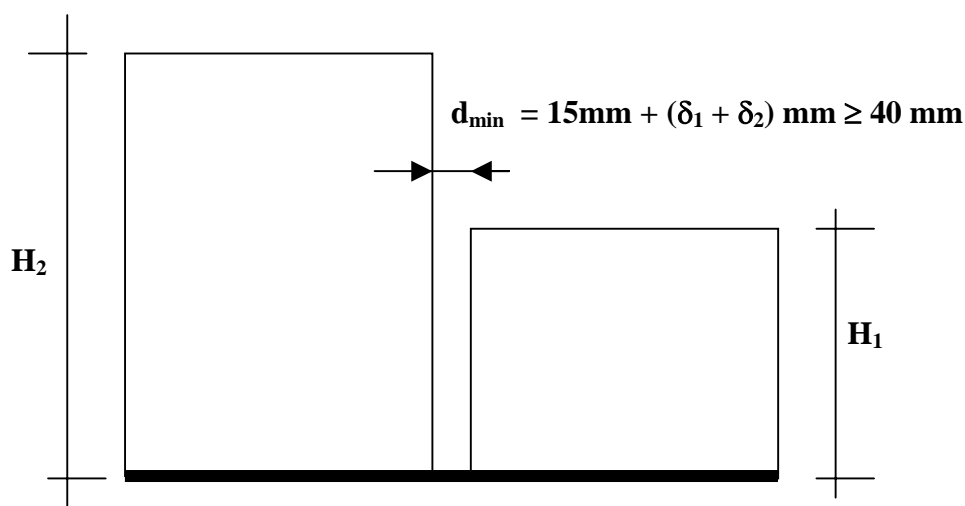
Figure 5.1 : Minimum width of seismic joint
