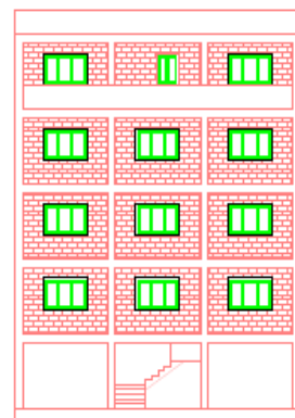
Figure 2. Front elevation.
