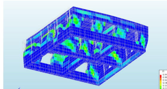
Figure 13. Stresses on stone masonry wall with seismic bands
