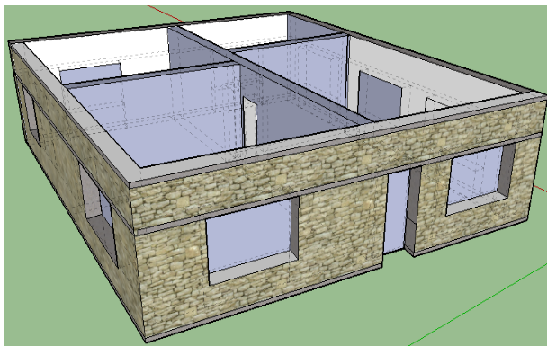
Figure 3. Stone Masonry with seismic bands
