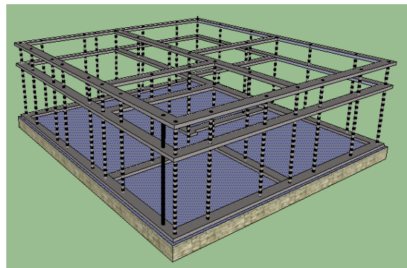
Figure 4. Seismic bands layout details
