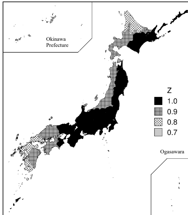
Figure 5.5-3: Earthquake Region Coefficient
