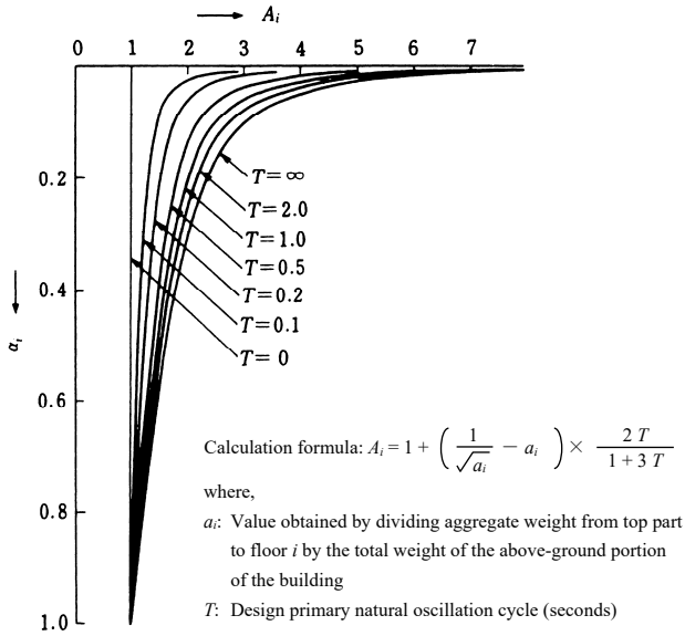
Figure 5.5-6: Distribution Factor of Seismic Layer Shear Force Coefficient
