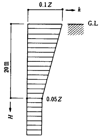
Figure 5.5-2: Horizontal Seismic Intensity Distribution in Underground Portion of a Building
